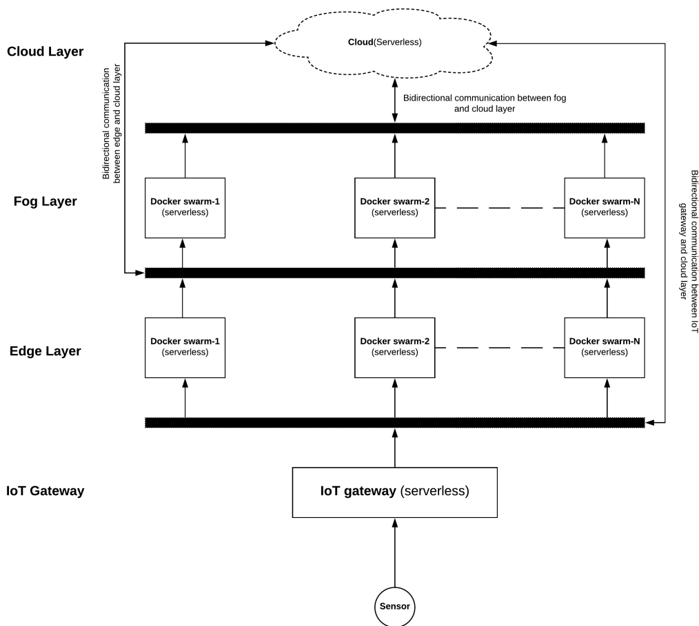
Figure 11. Communication for the function execution offloading
