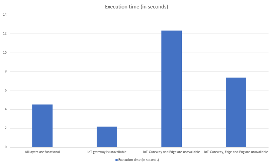
Figure 16. Function execution time in case of unavailability of the layers
