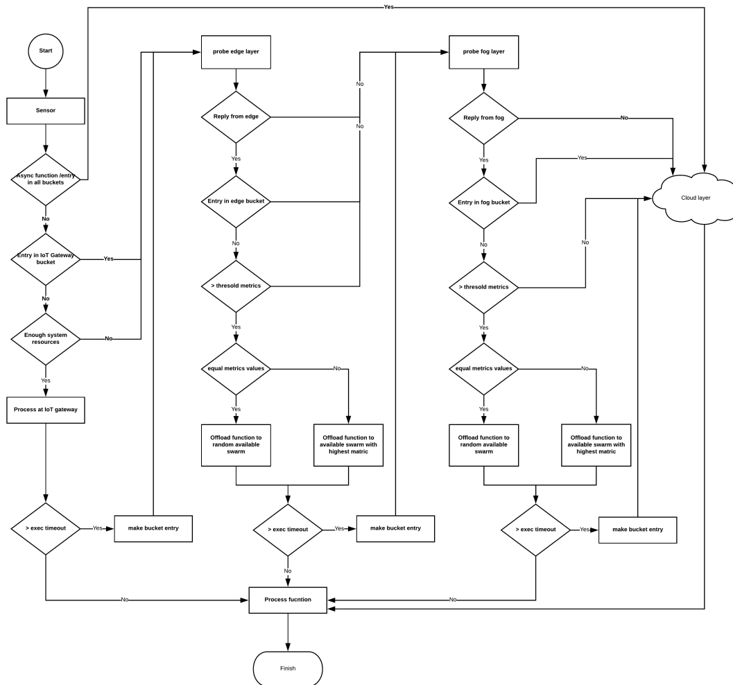
Figure 12. Function execution offloading flow diagram
