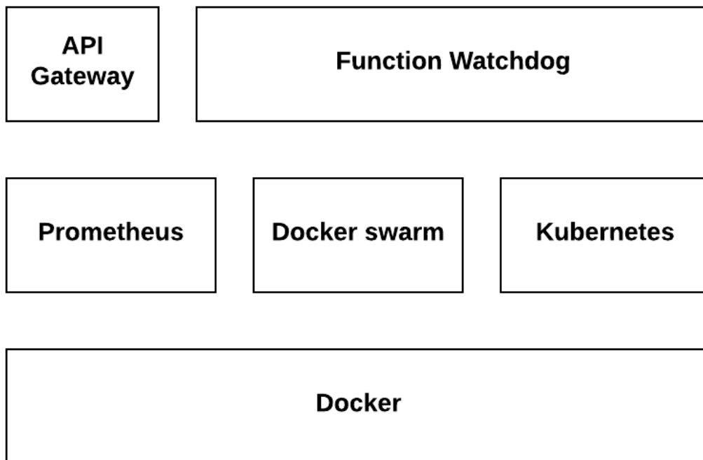
Figure 9. OpenFaaS components
