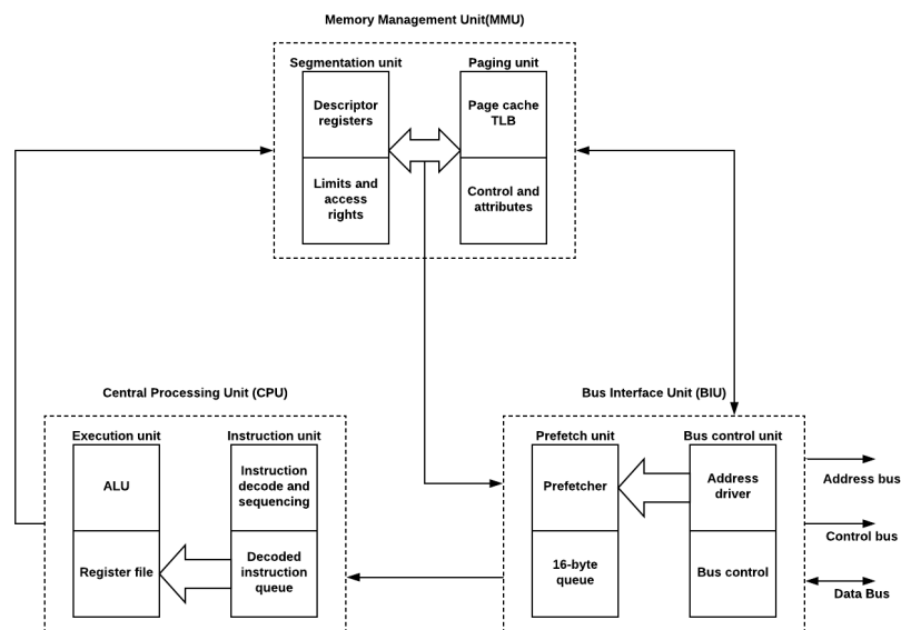
Figure 3. Intel 80386 internal architecture
