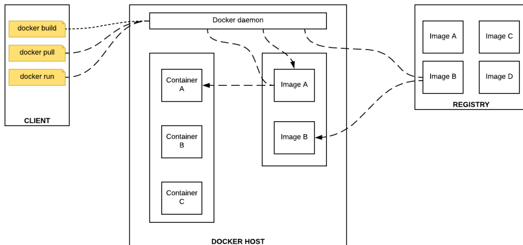
Figure 6. Docker architecture
