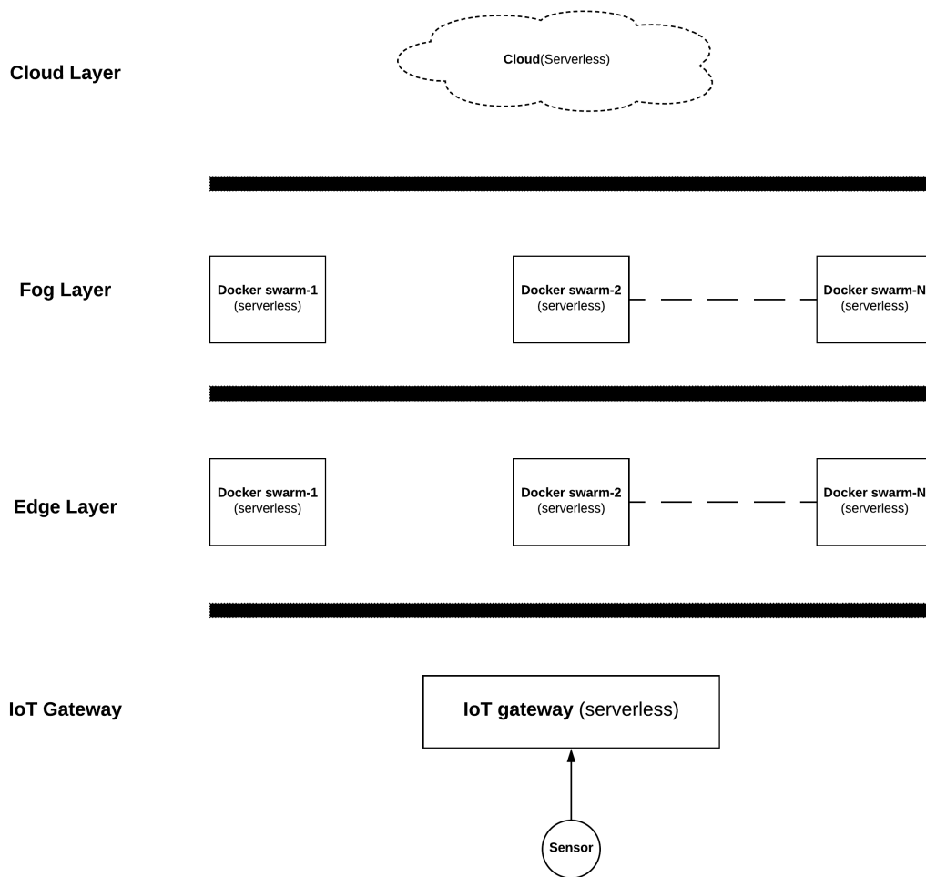
Figure 10. Multi-layered architecture
