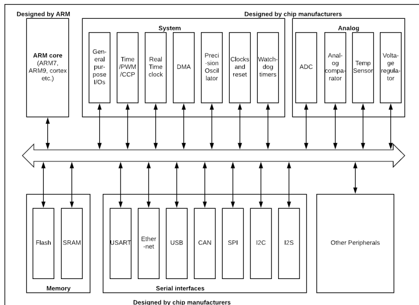
Figure 2. ARM simplified block diagram system on chip
