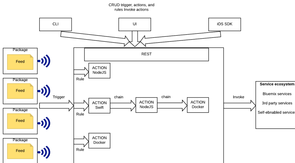
Figure 7. OpenWhisk high-level overview
