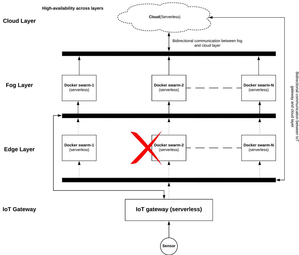
Figure 14. High availability across layers
