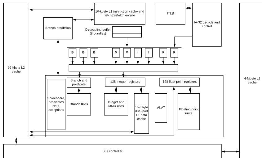
Figure 4. x64 architecture
