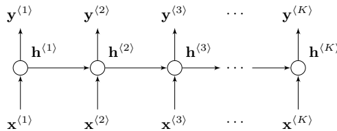
Fig. 3: Recurrent Neural Network
