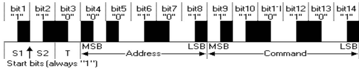
Figure 12. Example pulse stream of a RC-5 encoded message [27].
