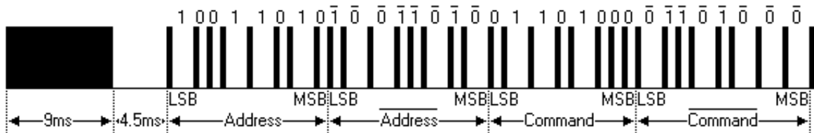
Figure 11. Example pulse stream of a NEC encoded message [26].
