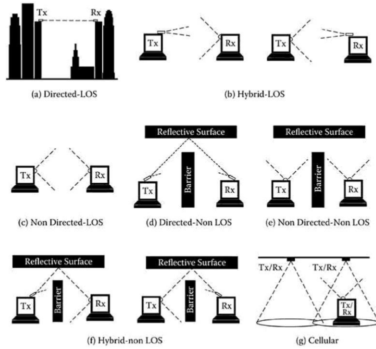
Figure 14. Different configurations of wireless IR links [29].
