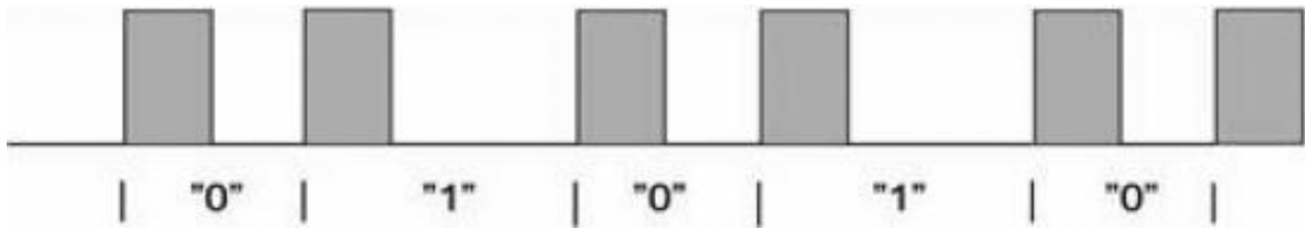
Figure 7. Pulse-distance coding [19].
