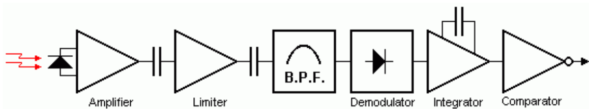
Figure 6. A typical block diagram of an IR receiver [21].
