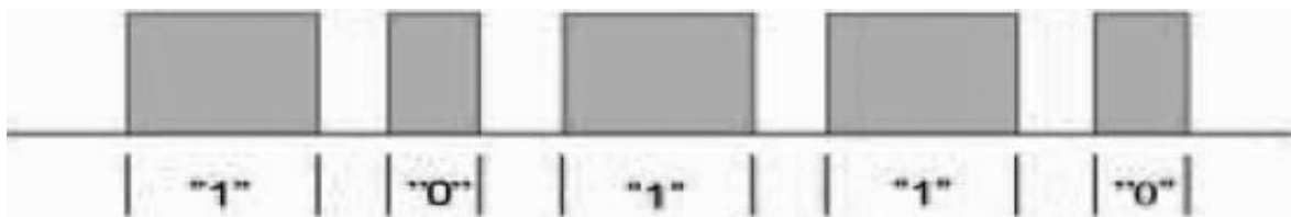
Figure 9. Pulse-length coding [19].
