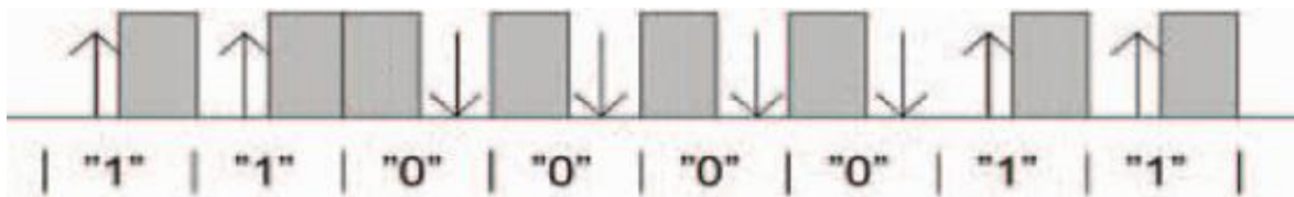
Figure 8. Manchester coding [19].
