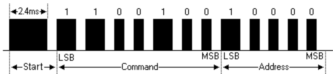
Figure 10. Example pulse stream of a 12-bit SIRC encoded message [25].
