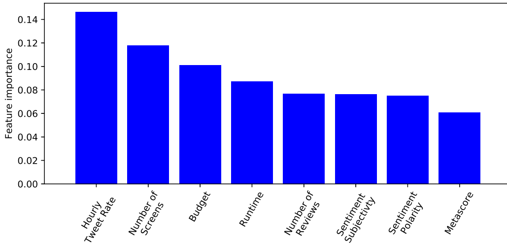
Figure 15. Feature importance for the Hollywood XGB* model in Table 10
