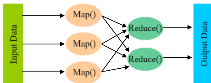
Figure 1: MapReduce process.
